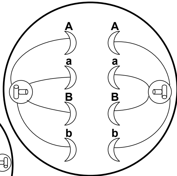
Anaphase
