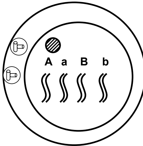
Anaphase
