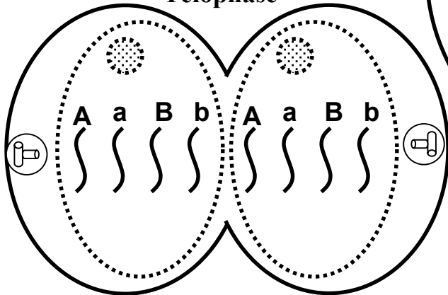
Telophase
