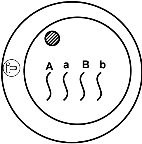
Early Interphase (G 1 )
